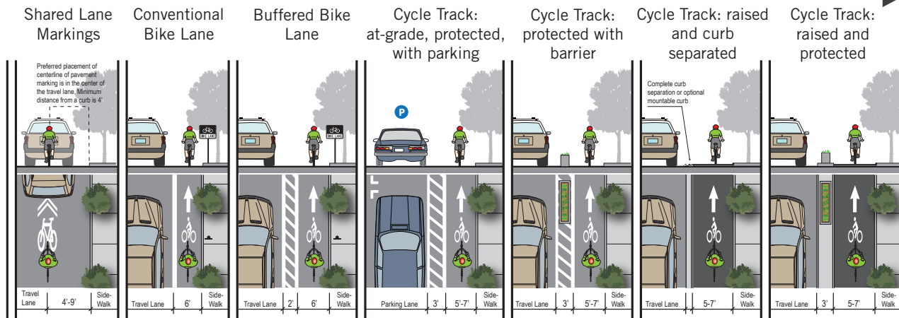
Figure 3. On-street bikeway continuum
