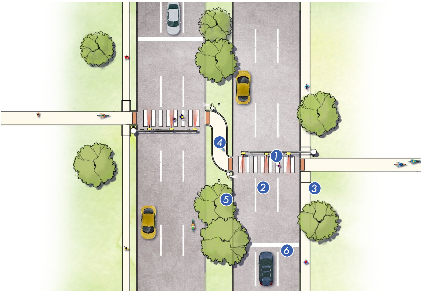
Typical HAWK Crossing Configuration
