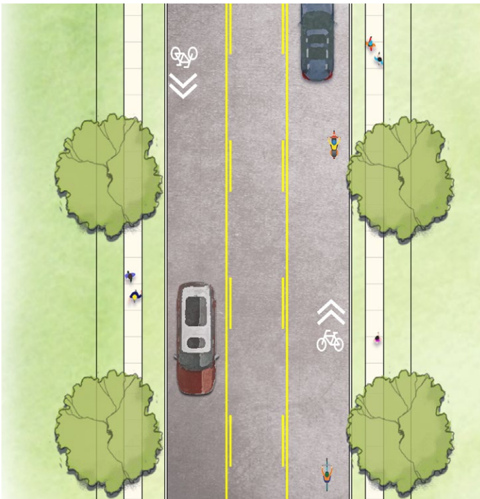
Shared Use Lane Markings
