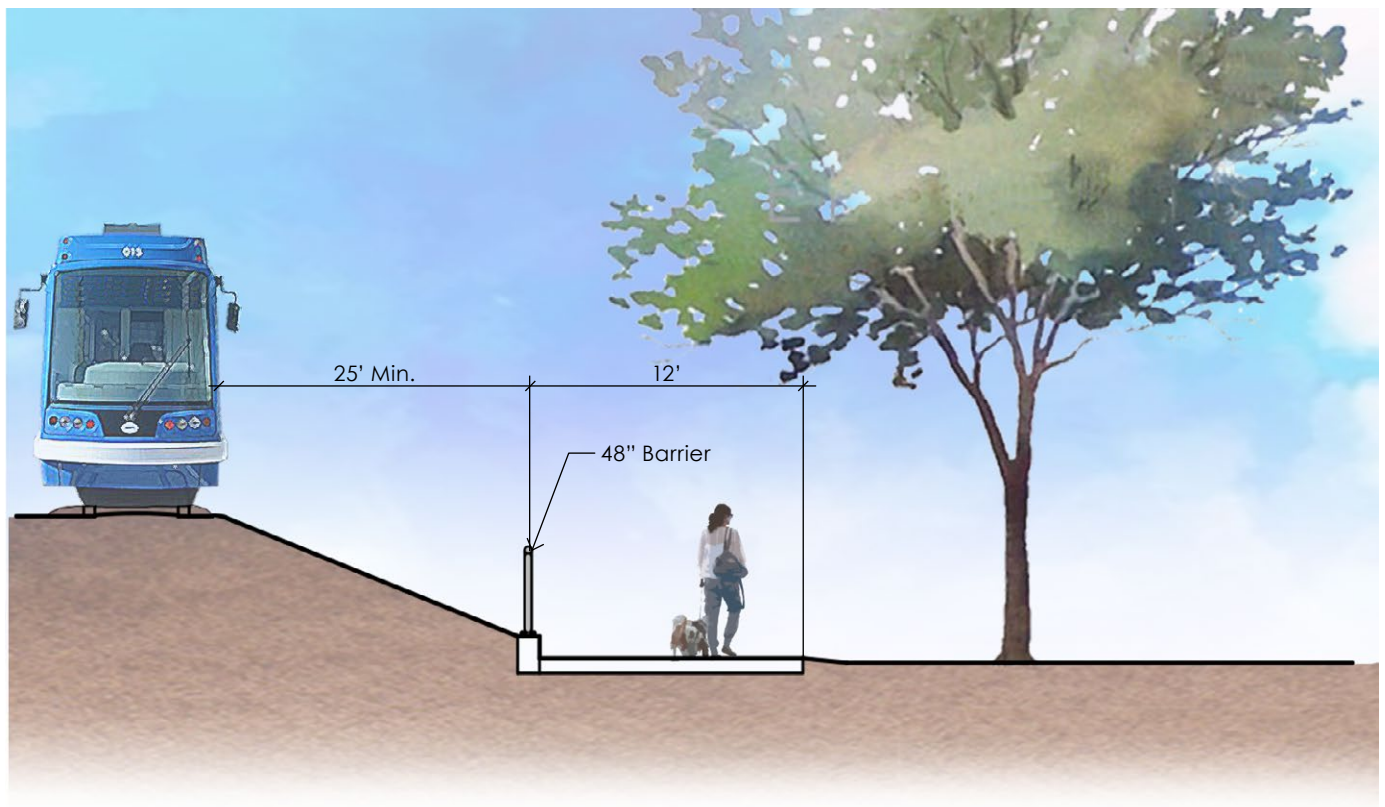
Typical Trail in Rail R.O.W.
