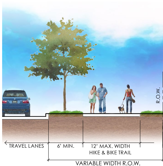
Trail in Right of Way
