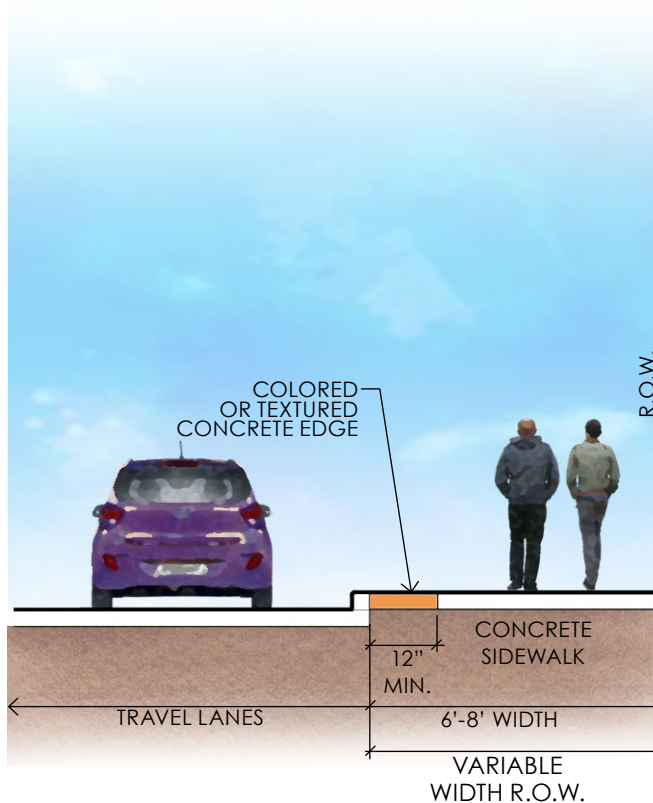
Widened Sidewalk with Contrasting Band
