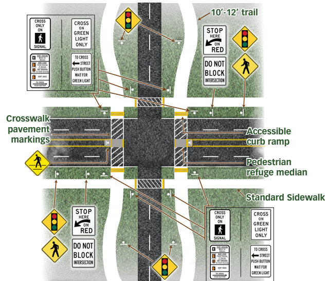
FIGURE 4.10 | SIGNALIZED TRAIL CROSSING AT ROADWAY INTERSECTION
