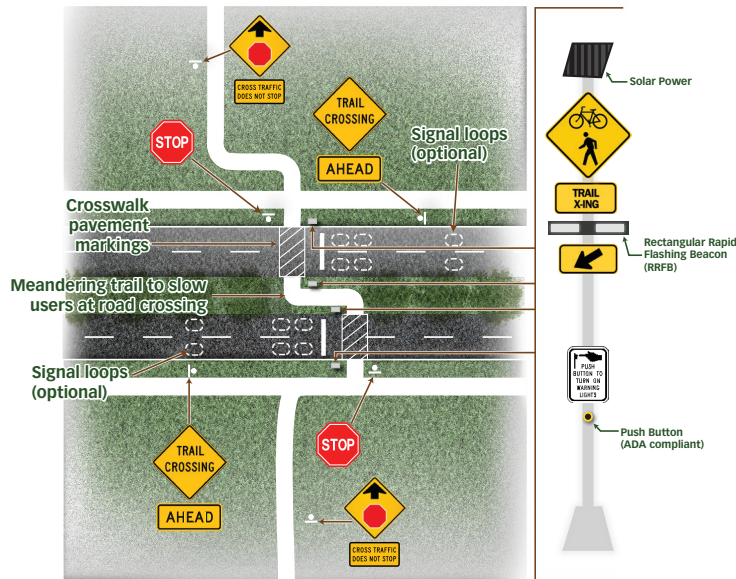
FIGURE 4.9 | SIGNALIZED TRAIL CROSSING TREATMENT (MID-BLOCK)
