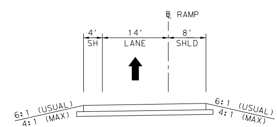
PROPOSED TYPICAL SECTION RAMP
