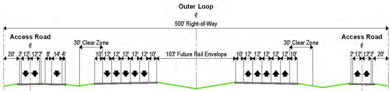
Figure 2. Collin County Outer Loop Ultimate Typical Cross Section
