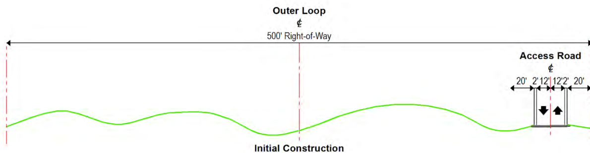
Figure 3. Segment 3a Initial Typical Section
